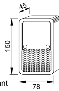
L2 Public Side Loudspeaker 40.006.112
