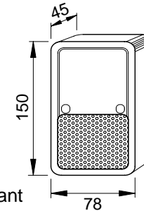
L2 Public Side Loudspeaker 40.006.112
